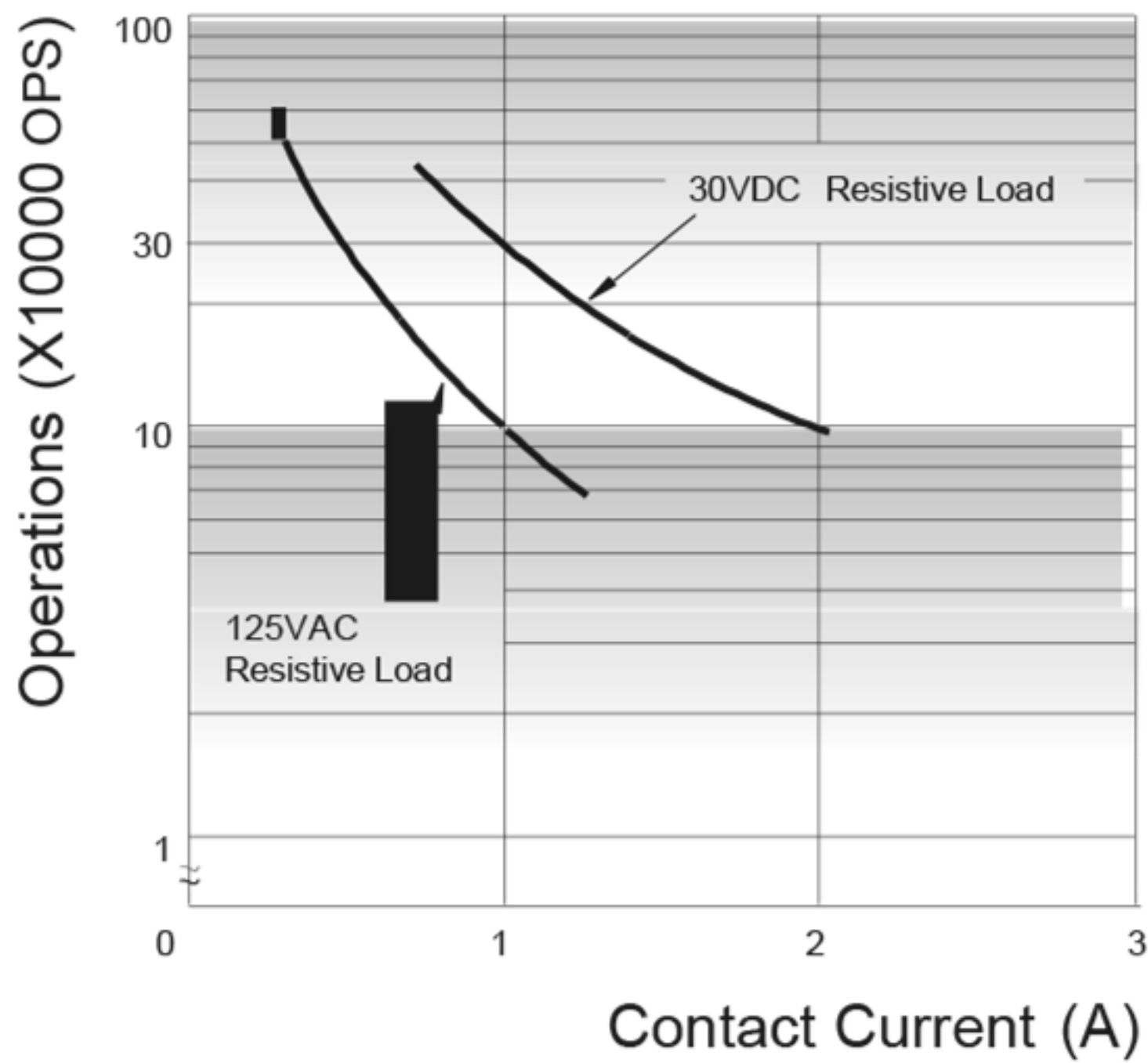
ENDURANCE CURVE
