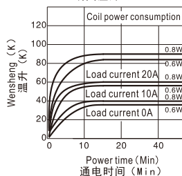
Coil temperature rise (at 23°C) 线圈温升 (at 23°C)
