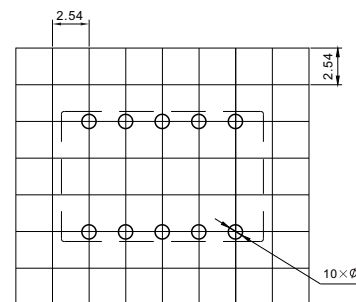
Tolerance:±0.1 Mounting (Bottom view)
